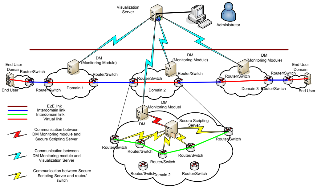
Figure 2: Ethernet Module Architecture
