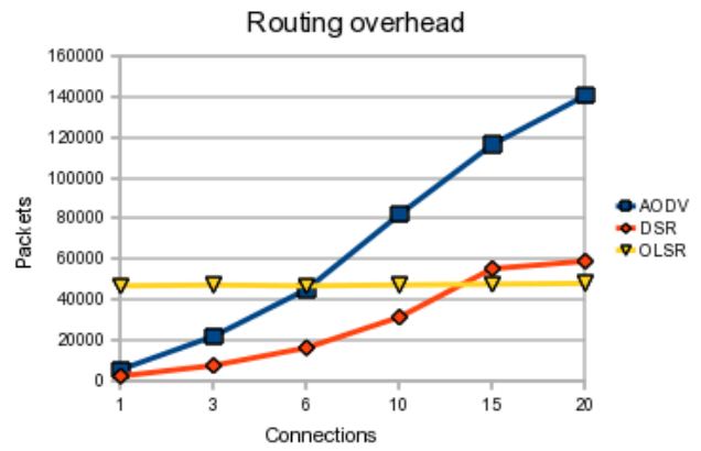
Figure 4. Routing overhead
