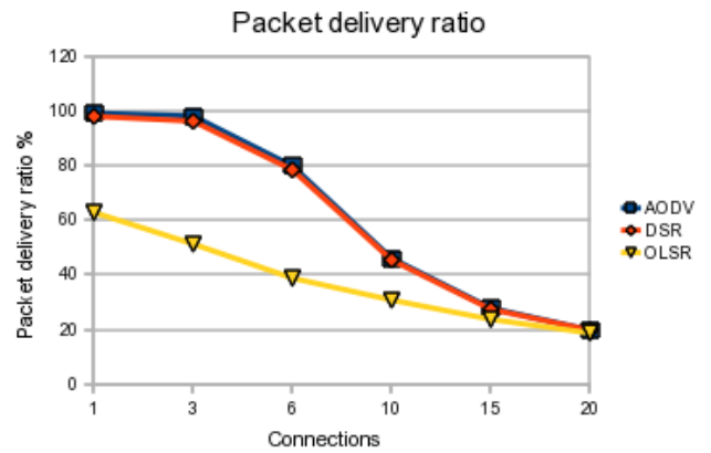
Figure 1. Delivery ratio over different maximum connections
