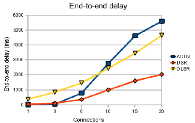
Figure 2. Average end to end delay (measured in milliseconds)
