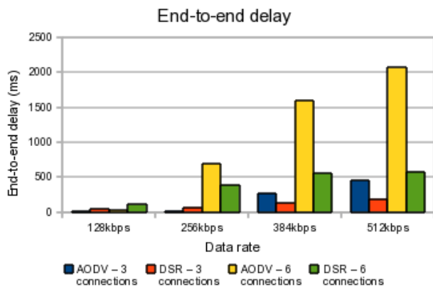
Figure 6. Average end to end delay over different data rates
