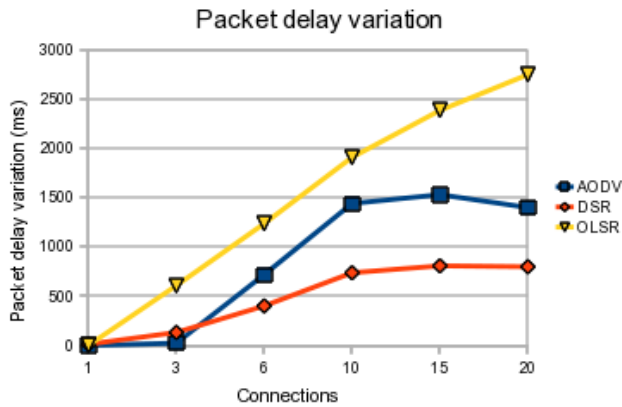
Figure 3. Packet delay variation (jitter)
