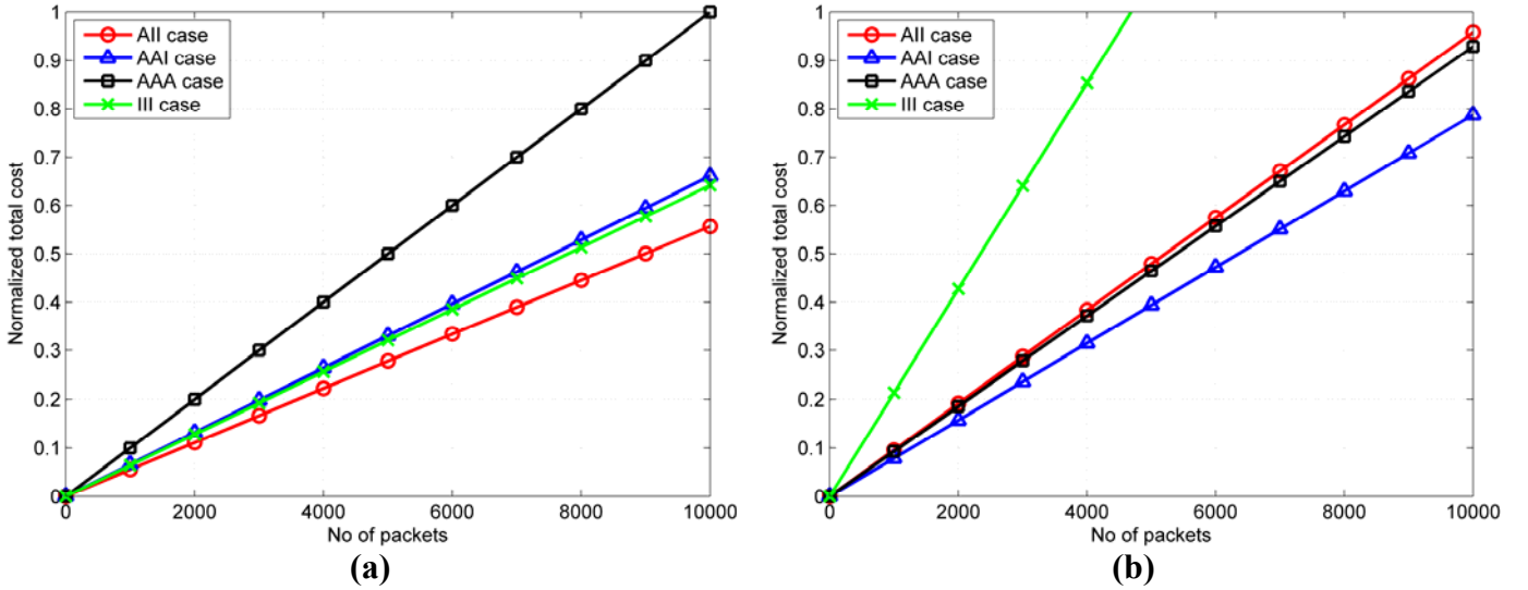
Figure 5. MBSFN cost for AII, AAI, AAA vs. number of packets for macro Case 1 when k_{air} = 0.9 and (a) UE drop location cells = 7, (b) UE drop location cells = 91.
