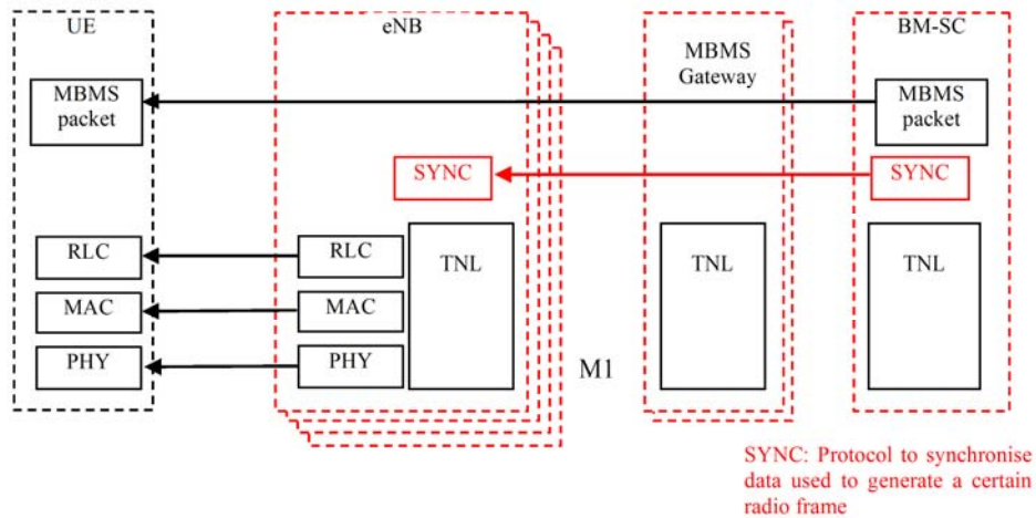
Figure 4. Content synchronization in MBSFN.
