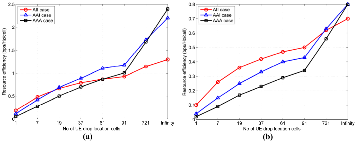
Figure 3. Resource efficiency vs. number of UE drop location cells for: (a) ISD = 500m (macro Case 1), (b) ISD = 1732m (macro Case 3).
