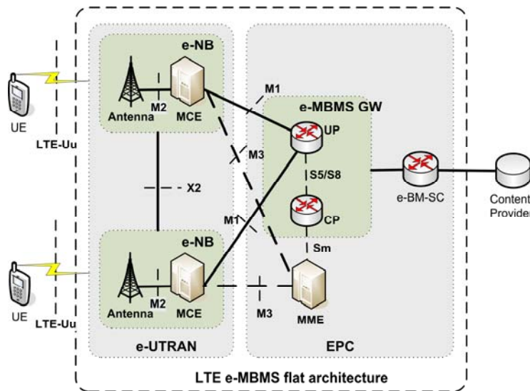
Figure 1. LTE e-MBMS flat architecture [3].
