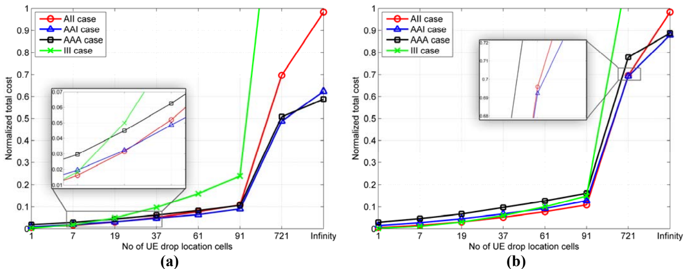
Figure 6. MBSFN cost for AII, AAI, AAA vs. number of UE drop location cells when k_{air} = 0.9 for: (a) ISD = 500m (macro Case 1), (b) ISD = 1732m (macro Case 3).
