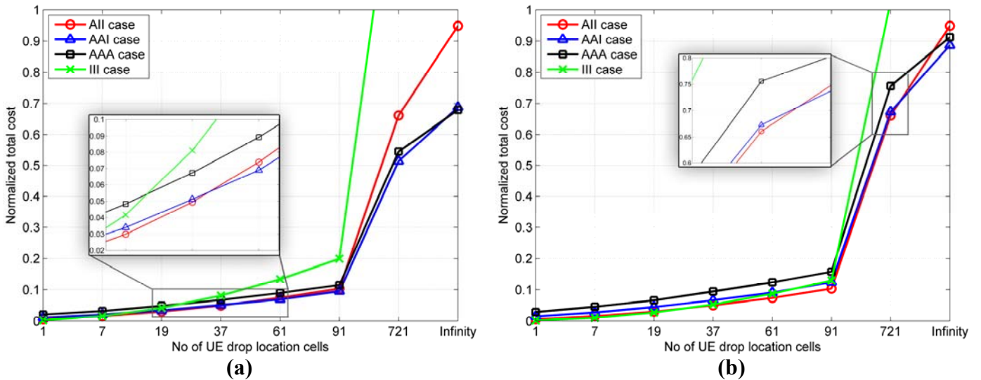
Figure 8. MBSFN cost for AII, AAI, AAA vs. number of UE drop location cells when k_{air} = 0.7 for: (a) ISD = 500m (macro Case 1), (b) ISD = 1732m (macro Case 3).
