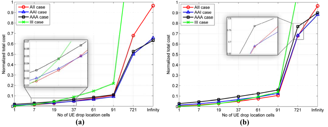
Figure 7. MBSFN cost for AII, AAI, AAA vs. number of UE drop location cells when k_{air} = 0.8 for: (a) ISD = 500m (macro Case 1), (b) ISD = 1732m (macro Case 3).
