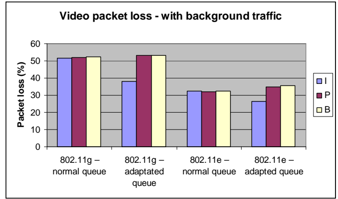
Figure 4. Video frame loss with background traffic
