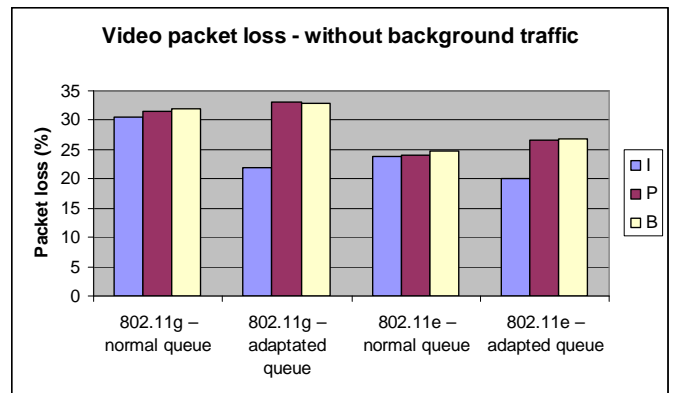
Figure 2. Video frame loss without background traffic
