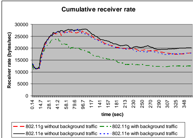
Figure 6. Cumulative receiver rate for video transmission
