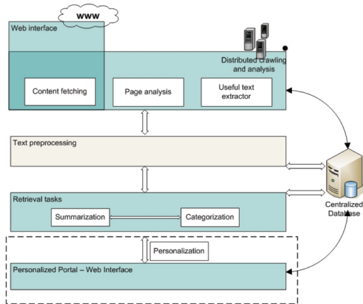
Figure 3: PeRSSonal's architecture
