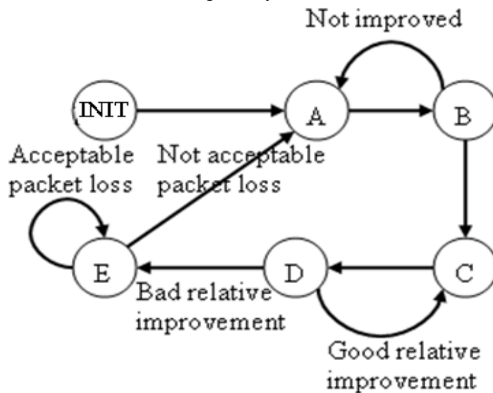
Figure 1. Finite automaton for the proposed mechanism for the sender.
