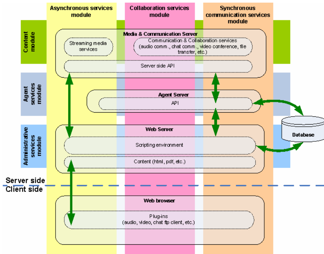
Figure 2: Integrated system architecture
